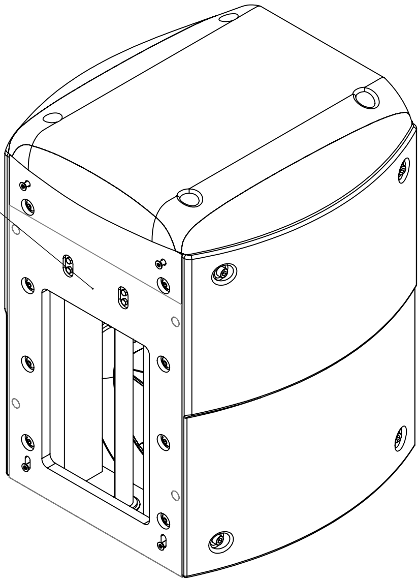
Drilling Template
